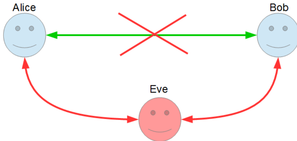
Abbildung 6: Man-in-the-middle
