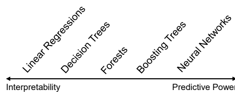
Fig. 6.2.: Example for interpretability vs predictive power by Hassani et al. [148].
